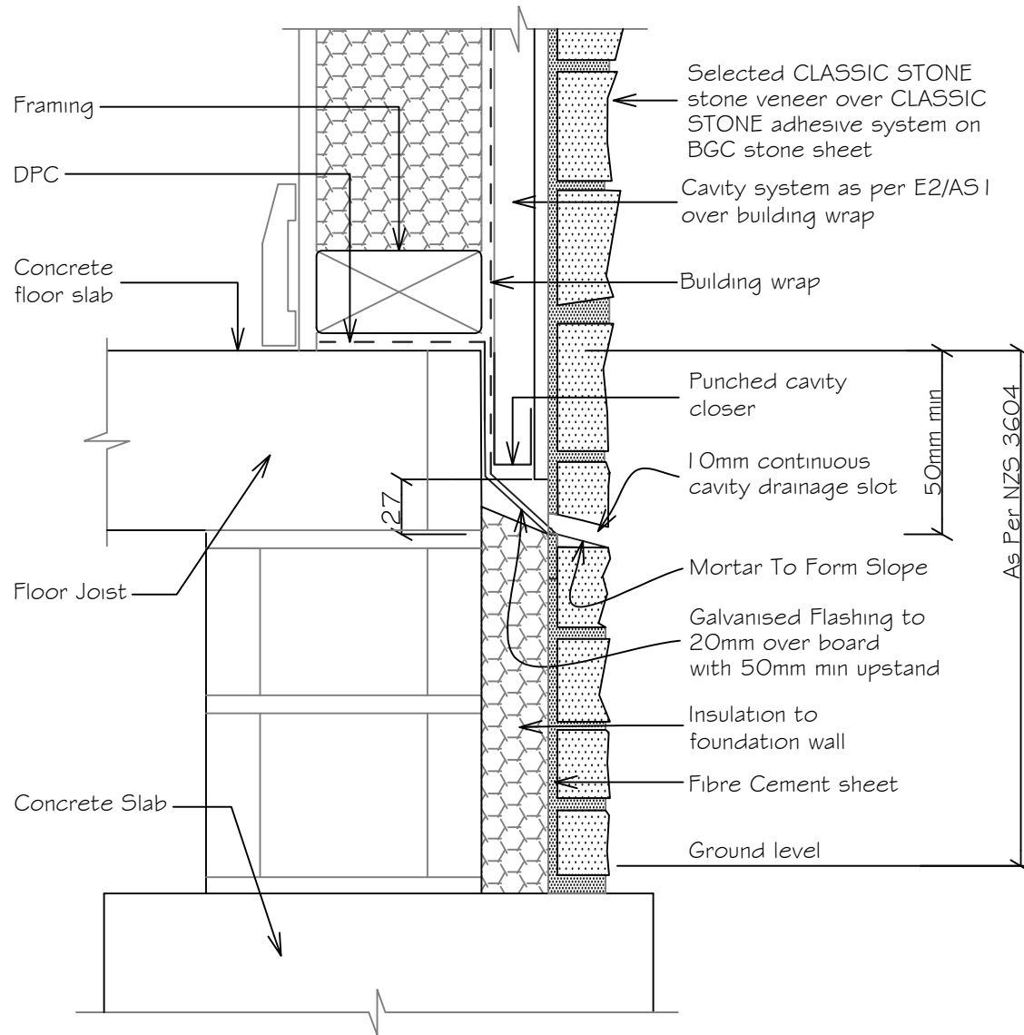
9b - Typical Slab Edge Detail (with continuous drainage slot)
